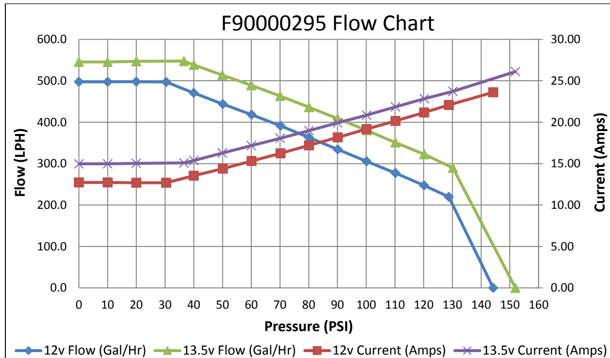
F90000295 No Check Valve: Flex Fuel Racing Pump
