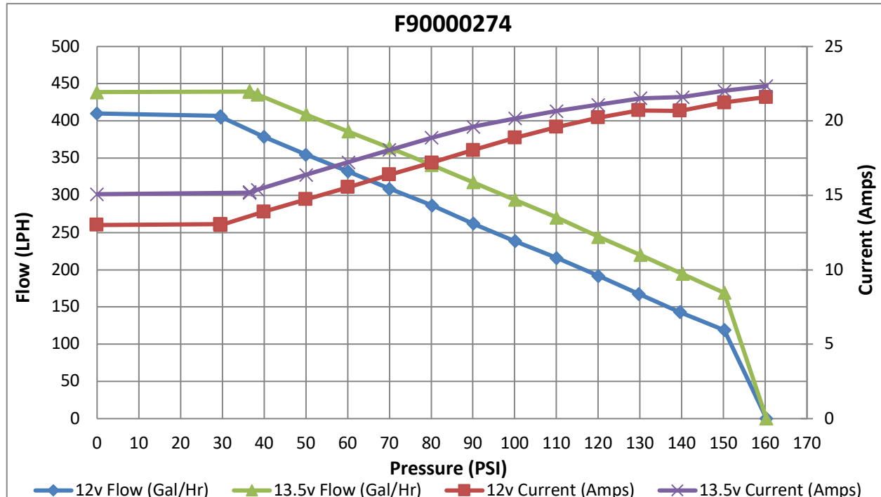
F90000274: 400+LPH Flex Fuel Pump
